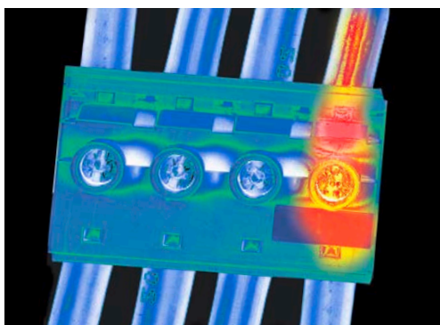
Overload of the neutral conductor
