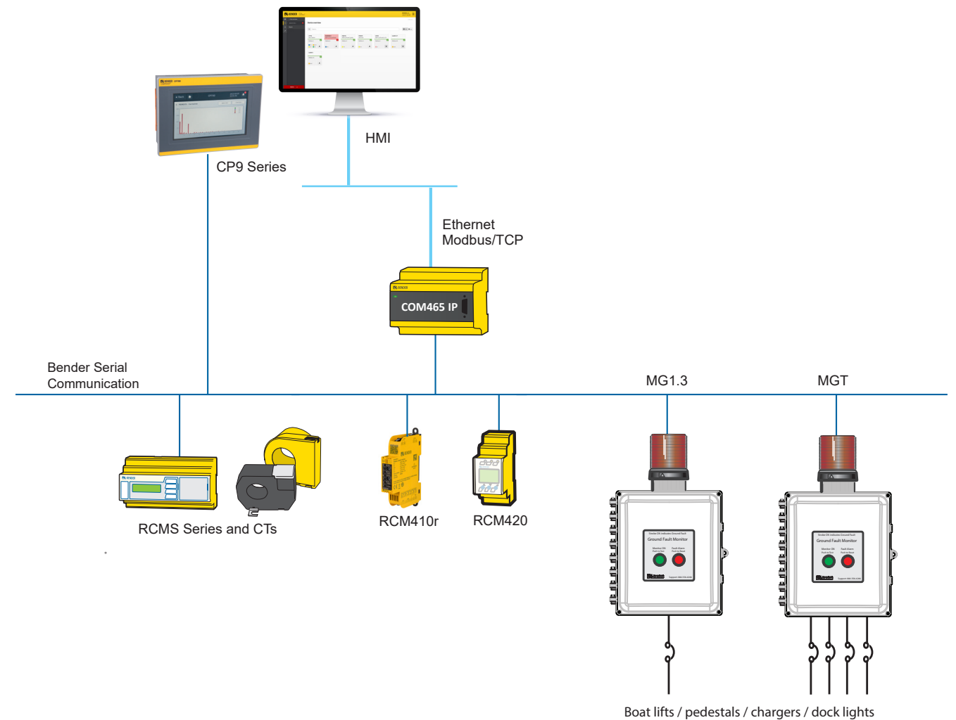
Drawing: Marina communications and centralized branch monitoring with MarinaGuard
